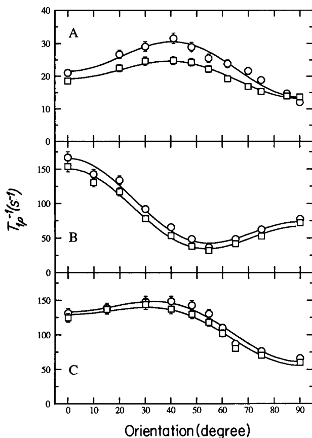
FIGURE 3 The orientation dependence of ^{19}\text{F} T_{1\rho}^{-1} for oriented bilayers: (A) pure 2-[7,7- ^{19}\text{F}_2 ]DMPC- \text{d}_{52} ; (B) 2-[7,7- ^{19}\text{F}_2 ]DMPC- \text{d}_{52} with 12 wt% cholesterol; and (C) 2-[7,7- ^{19}\text{F}_2 ]DMPC- \text{d}_{52} with 14 wt% gramicidin. (O) H_1 = 2 Gauss; ( \square ) H_1 = 4 Gauss. Solid lines represent the best theoretical fits using the equations from Table 2. Note that B and C have a different vertical scale than A.
