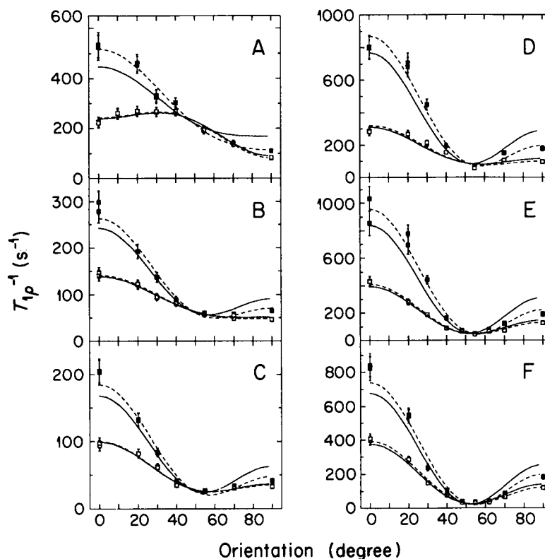
FIGURE 5 The orientation dependence of ^{19}\text{F} T_{1\rho}^{-1} for oriented bilayers: (A) 2-[4,4- ^{19}\text{F}_2 ]DMPC with 10 wt% gramicidin; (B) 2-[8,8- ^{19}\text{F}_2 ]DMPC with 10 wt% gramicidin; (C) 2-[12,12- ^{19}\text{F}_2 ]DMPC with 10 wt% gramicidin; (D) 2-[4,4- ^{19}\text{F}_2 ]DMPC with 10 wt% cholesterol; (E) 2-[8,8- ^{19}\text{F}_2 ]DMPC with 10 wt% cholesterol; and (F) 2-[12,12- ^{19}\text{F}_2 ]DMPC with 10 wt% cholesterol. Solid lines are the best fits using the equations given in Table 2, whereas dashed lines represent fits obtained when including a ^{19}\text{F} - ^1\text{H} cross-polarization term. (■) H_1 = 2 Gauss; (□) H_1 = 4 Gauss. Note that the vertical scale in each panel may be different.
